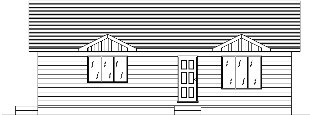
FRONT ELEVATION
